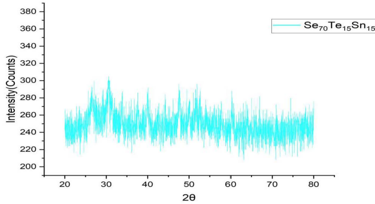
Figure 4. X-ray diffraction pattern of \text{Se}_{70}\text{Te}_{15}\text{Sn}_{15} .
