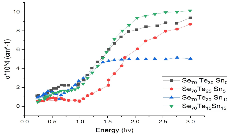
Figure 5. Absorption coefficient ( \alpha ) against photon energy in \text{Se}_{70}\text{Te}_{30}\text{Sn}_{30-x} thin films.
