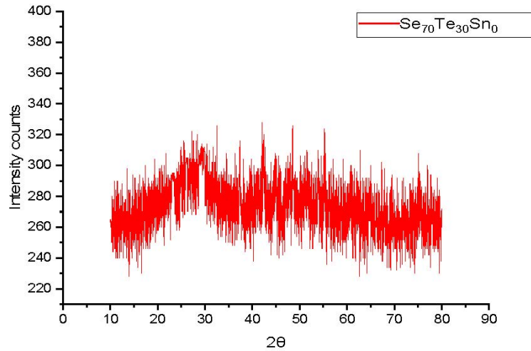
Figure 1. X-ray diffraction pattern of Se 70 Te 30 Sn 0 .
