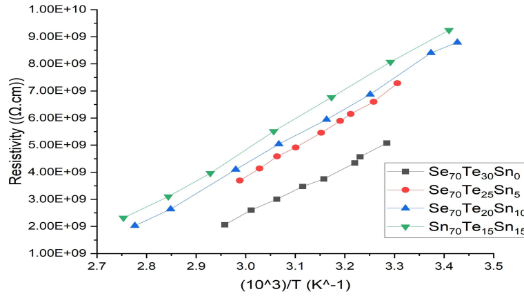
Figure 6. Temperature dependence of resistivity.
