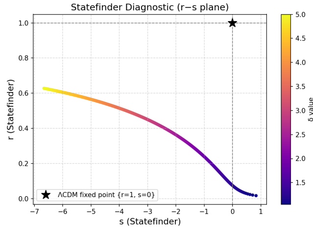
Figure 7. Statefinder r-s diagnostic plane, parametrised by \delta (colour scale). The \Lambda CDM fixed point \{r, s\} = \{1, 0\} is marked by a star. The present f(R, \mathcal{L}_m) BIII model traces a trajectory clearly distinct from \Lambda CDM, quintessence ( s > 0, r < 1 ), and Chaplygin gas ( s < 0, r > 1 ) [21], providing a geometric observational discriminator. A similar statefinder analysis for f(R, \mathcal{L}_m) FLRW models was reported in [10, 11].
