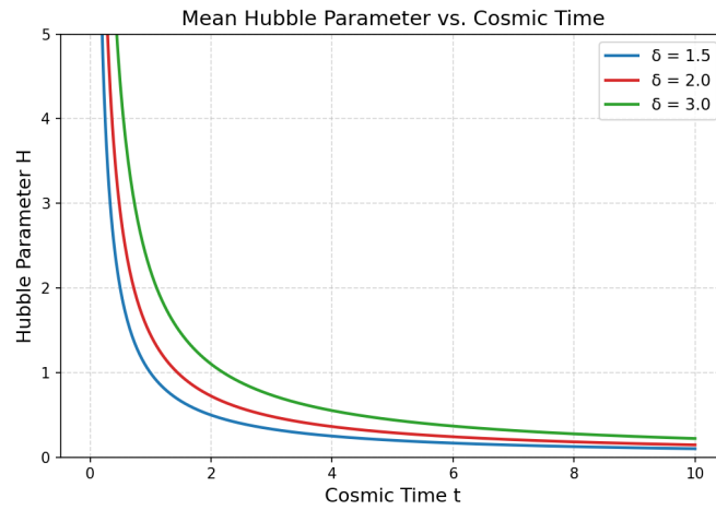
Figure 3. Mean Hubble parameter H vs. t . H is a monotonically decreasing function of time, diverging at the initial singularity t \rightarrow 0 and asymptotically approaching zero. The power-law decay H \propto t^{-1} mirrors results from anisotropic BIII f(R, T) models [19,20].
